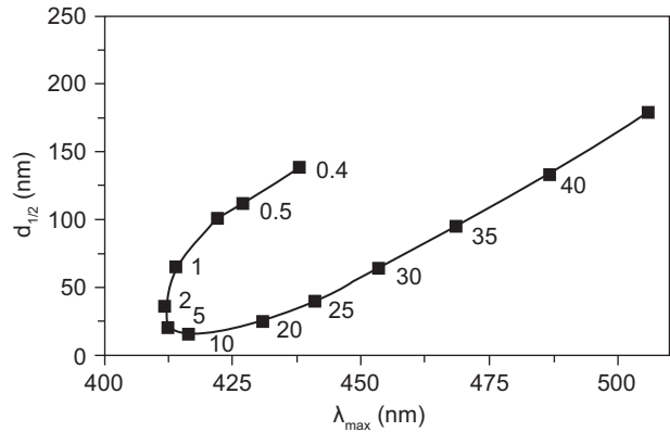
Figure 6. Determination of silver particle radius from \lambda_{max} and d_{1/2} [22].
