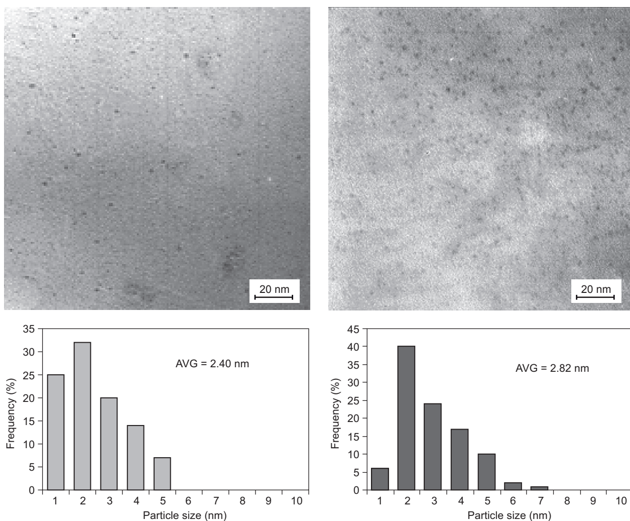
Figure 7. TEM Image and the particle diameter distribution of silver nanoparticles distributed in silica matrix after the heat-treatment at 500°C (left) and 550°C (right).
